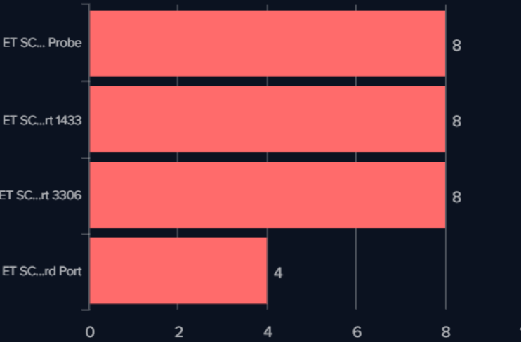
Top Suricata Signatures
